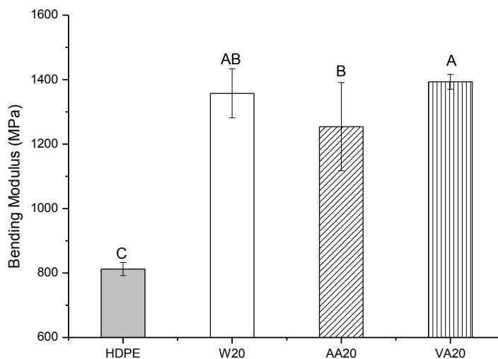
Fig. 8. Effect of acetylation on the flexural modulus values (b) of WPCs
