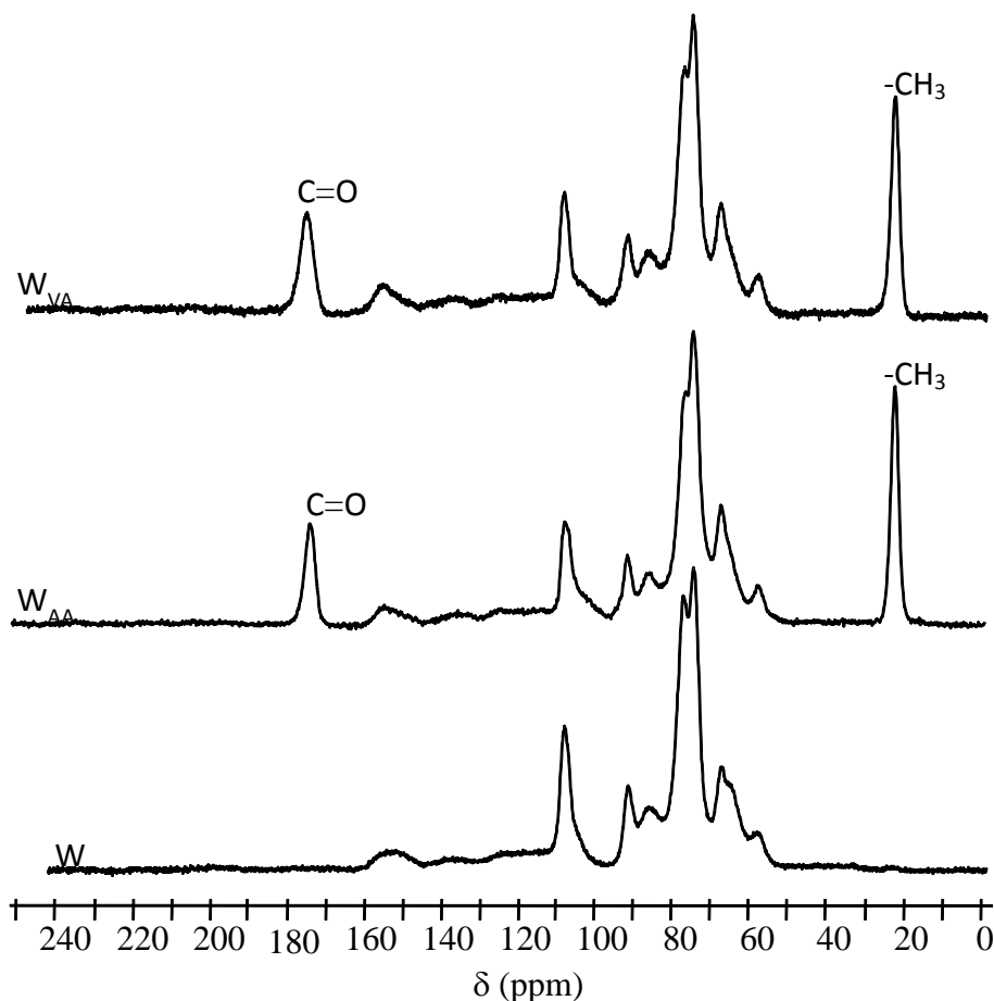
Fig. 3. 13 C CP-MAS NMR spectra of unmodified ( W ), acetic anhydride-modified (24% WPG) ( W_{AA} ), and vinyl acetate-modified (19% WPG) ( W_{VA} ) Scots pine wood flour
