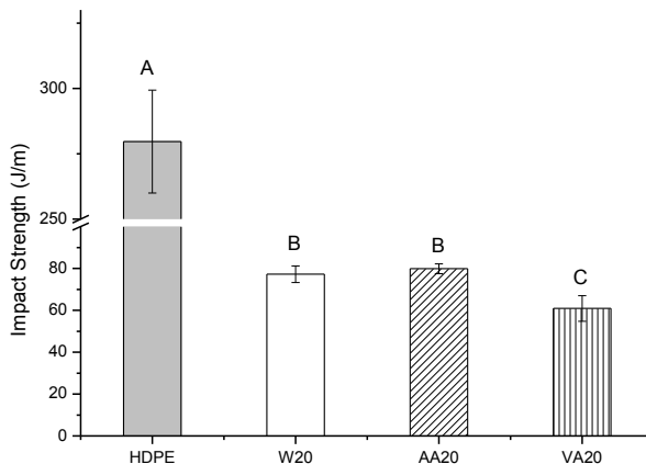
Fig. 10. Effect of acetylation on the impact strength (IS) values of WPCs
