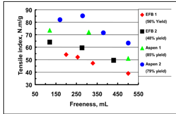
Fig. 13. Tensile index vs. freeness for EFB and aspen pulps (Law and Jiang 2001)
