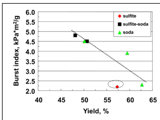
Fig. 11. Burst index vs. pulp yield of EFB pulps (Wanrosli et al. 1998)
