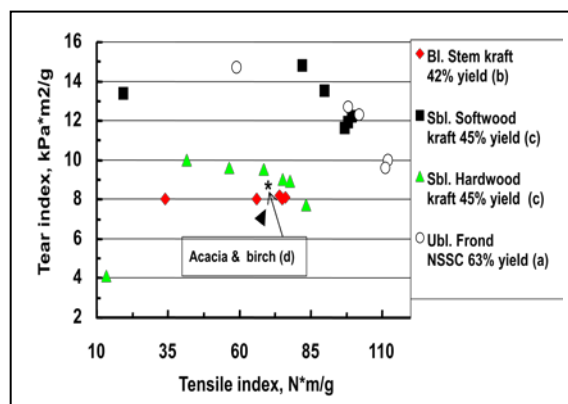
Fig. 7. Tear index vs. tensile index of oil palm and wood pulps
