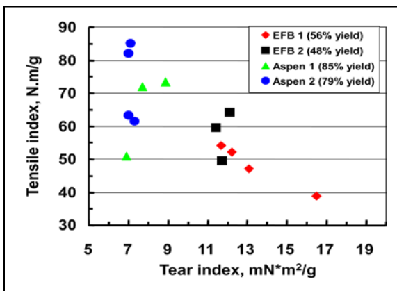
Fig. 16. Tensile index vs. tear index of EFB and aspen pulps (Law and Jiang 2001)
