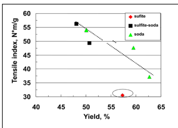
Fig. 10. Tensile index vs. pulp yield of EFB pulps (Wanrosli et al. 1998)
