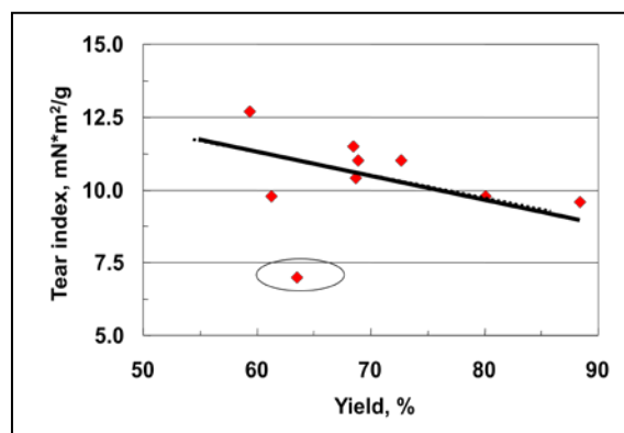
Fig. 9. Tear index vs. pulp yield of frond NSSC pulps (Yusoff 1997)
