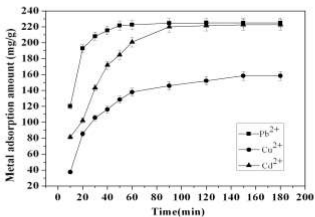
Fig. 6. The effect of contact time on adsorption of heavy metal ions
