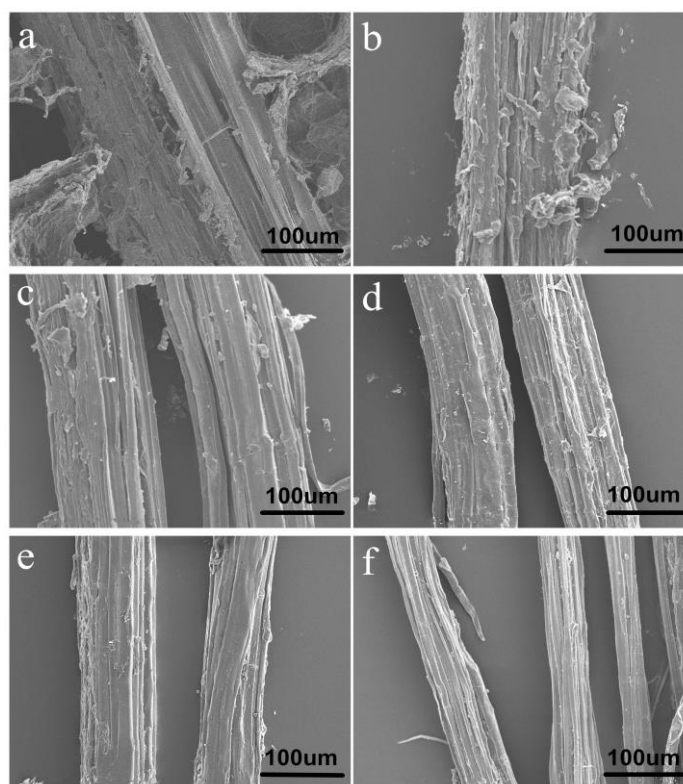
Fig. 4. SEM micrographs for (a) untreated bark of cotton stalks and CSBF by steam flash-explosion at the steam pressure of (b) 1.5 MPa, (c) 2.0 MPa, (d) 2.5 MPa, (e) 3.0 MPa, and (f) 3.5 MPa for 2 min
