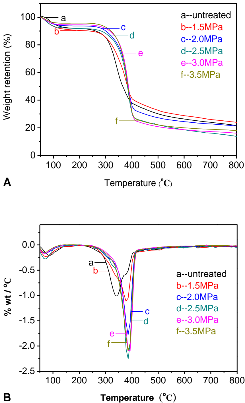
Fig. 9. (A) TG and (B) DTG curves for (a) untreated bark of cotton stalks and CSBF by steam flash-explosion at steam pressures of (b) 1.5 MPa, (c) 2.0 MPa, (d) 2.5 MPa, (e) 3.0 MPa, and (f) 3.5 MPa for 2 min
