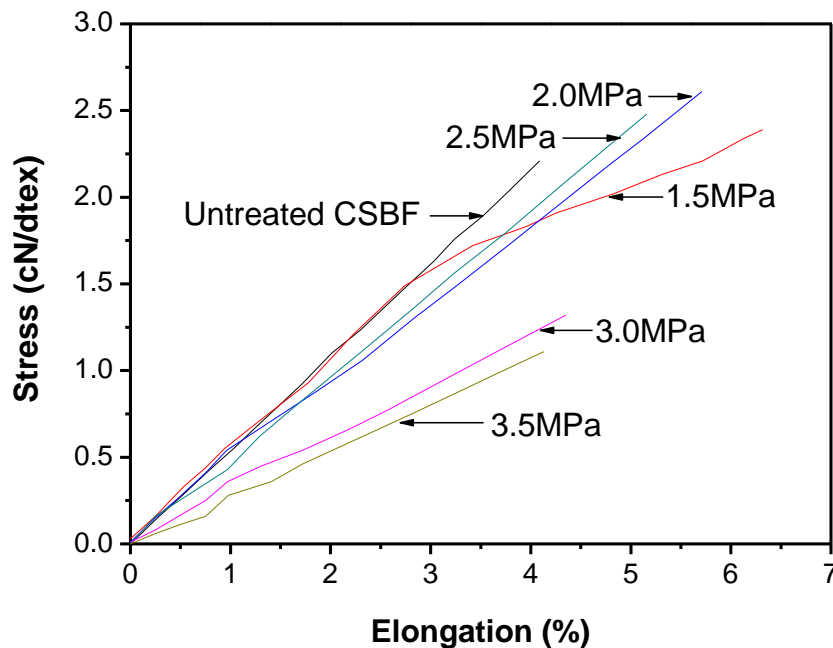
Fig. 7. Tensile stress-strain curves of untreated CSBF and CSBF by steam flash-explosion under different steam pressures from 1.5-3.5 MPa for 2 min
