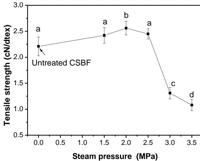
Fig. 6. Effect of steam pressure on tensile strength of CSBF by steam flash-explosion for 2 min. Note that the data points with different letters represent statistically significant differences ( p < 0.05 ). Data reported as mean \pm standard deviation
