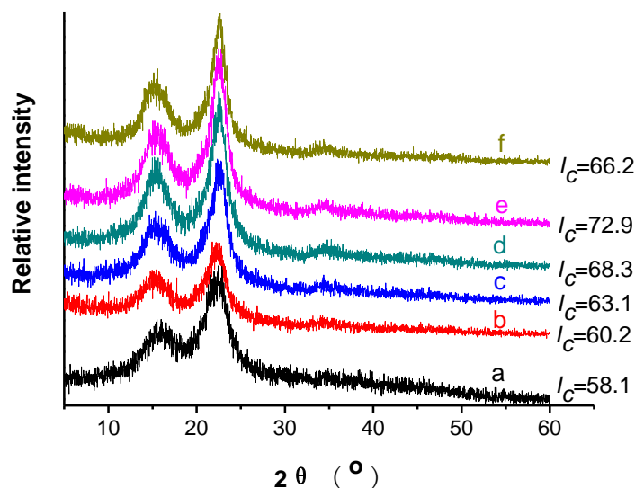
Fig. 2. X-ray diffraction curves and crystallinity index ( I_c ) for (a) untreated bark of cotton stalks and CSBF by steam flash-explosion under the steam pressures of (b) 1.5 MPa, (c) 2.0 MPa, (d) 2.5 MPa, (e) 3.0 MPa, and (f) 3.5 MPa for 2 min
