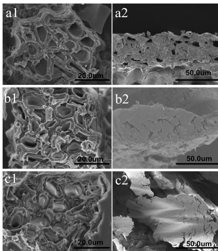
Fig. 8. SEM micrographs of (1) the fracture surfaces and (2) the cross-sections of (a) untreated bark of cotton stalks and CSBF by steam flash-explosion at steam pressures of (b) 2.5 MPa and (c) 3.5 MPa for 2 min
