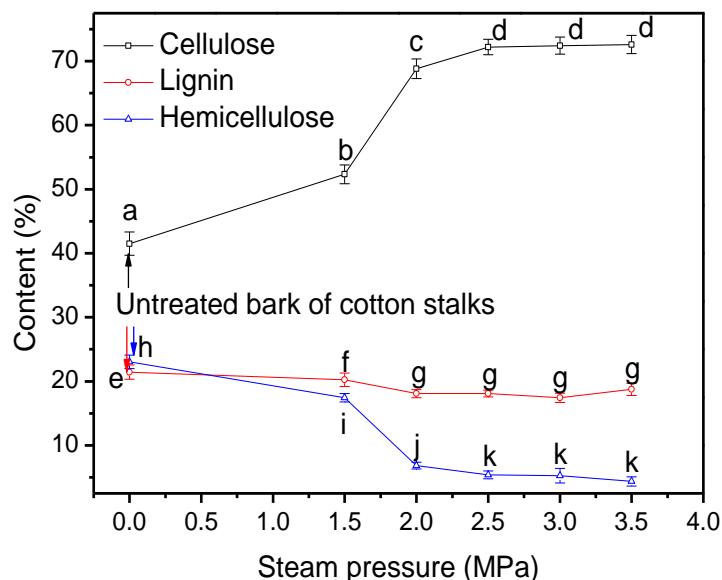
Fig. 1. Effect of steam pressure on constituent of CSBF by steam flash-explosion for 2 min. Note that data points with different letters represent statistically significant differences ( p < 0.05 ). Data reported as mean \pm standard deviation
