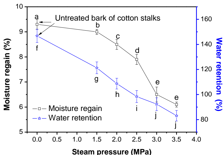
Fig. 5. Effect of steam pressure on moisture regain and water retention of CSBF by steam flash explosion for 2 min. Note that data points with different letters represent statistically significant differences ( p < 0.05 ). Data reported as mean \pm standard deviation
