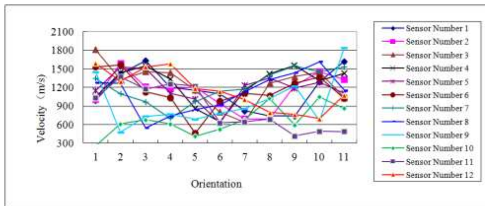
Fig. 9. The stress wave velocities of different orientations in sample 3
