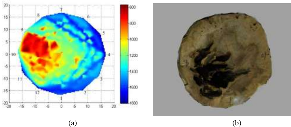
Fig. 11. Reconstruction tomogram and the photograph of the cross section of sample 3
