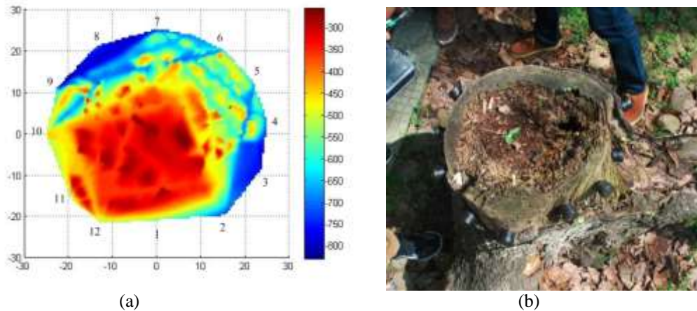
Fig. 8. The reconstruction tomogram and the photograph of the tree stump
