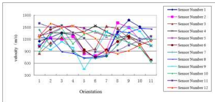
Fig. 3. Stress wave velocities of different orientations in standing tree of sample 1
