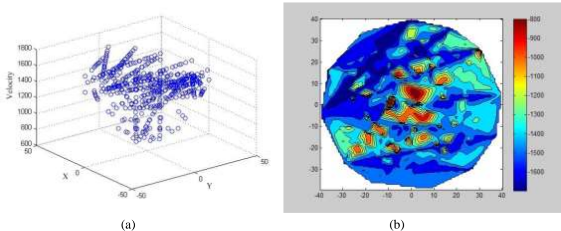
Fig. 4. Spatial distribution of the stress wave velocities and the contour map in standing tree of sample 1
