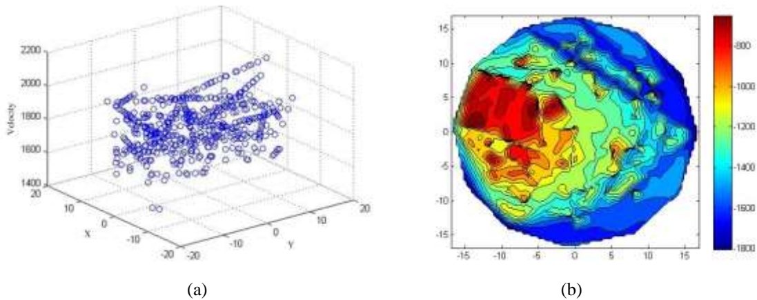
Fig. 10. Spatial distribution of stress wave velocity and the contour map of sample 3
