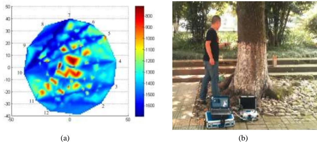
Fig. 5. The reconstruction tomogram and the testing photograph of the tree sample 1
