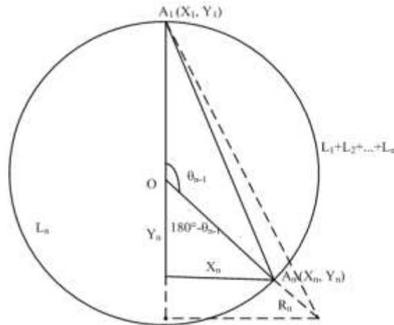
Fig. 1. Coordinate system of the receiving sensors.
