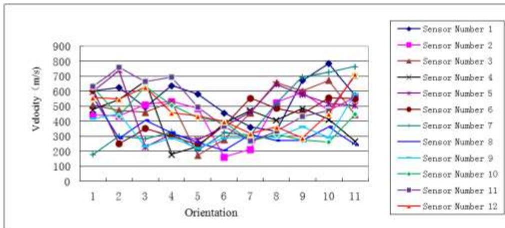
Fig. 6. Stress wave velocities of different orientations in tree stump of sample 2
