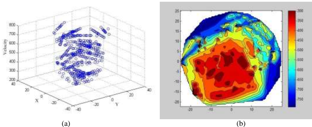
Fig. 7. Spatial distribution of stress wave velocity and the contour map in tree stump of sample 2
