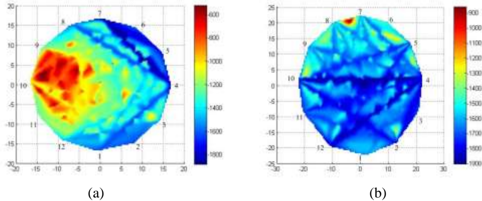
Fig. 12. The reconstruction tomograms of sample 3 in second measurements and sample 4
