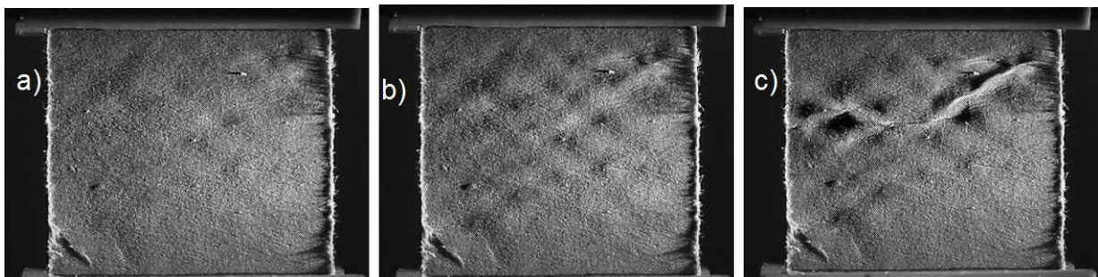
Figure 13. Excerpted time sequence video snapshots of a glancing angle illuminated ECT test of a 35-26C flute board: a), 5.7 kN/m load, 1.3% strain, some buckling is evident b), peak load 6.7 kN/m, 1.6% c), post failure 4.5 kN/m, 2.1% , crease forms joining micro-plate buckling crests
