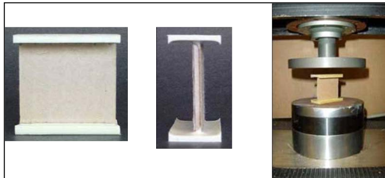
Figure 3. An ECT sample embedded in supporting epoxy resin strips front and side views and (right) mounted between the platens of a compression tester
