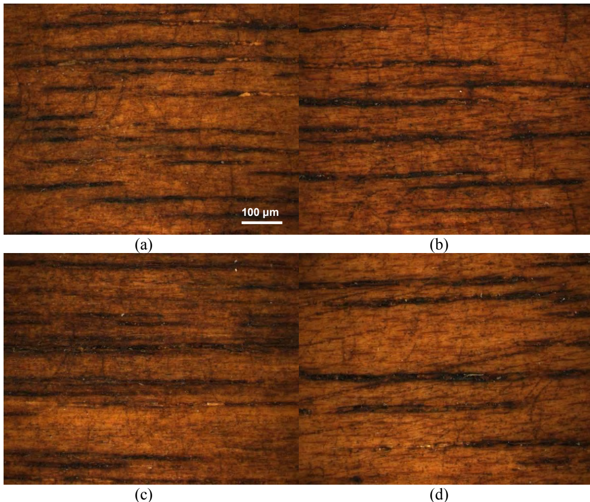
Fig. 2. Images of stained surfaces (a) lumber with a water-based stain; (b) lumber with a solvent-based stain; (c) veneer with a water-based stain; (d) veneer with a solvent-based stain
