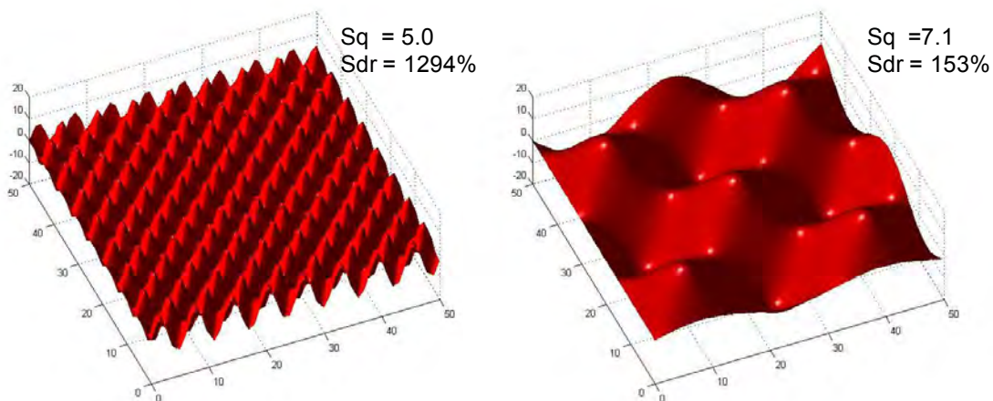
Fig. 1. Comparison of roughness parameters for two hypothetical surfaces
