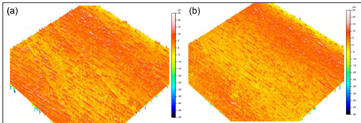
Fig. 8. 3D Renderings of profilometric measurements on edge-glued yellow birch panels (a) with a water-based stain (b) with a solvent-based stain. Color scale goes from -50 \mu\text{m} to 25 \mu\text{m} Surface dimensions: 20 x 20 mm
