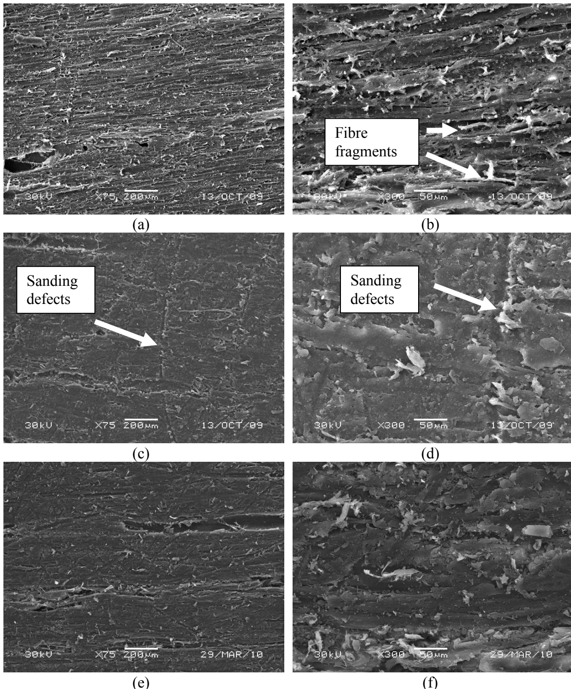
Fig. 6. Veneer samples stained with a water-based stain (a, b); solvent-based stain (c, d) and untreated samples (e, f)
