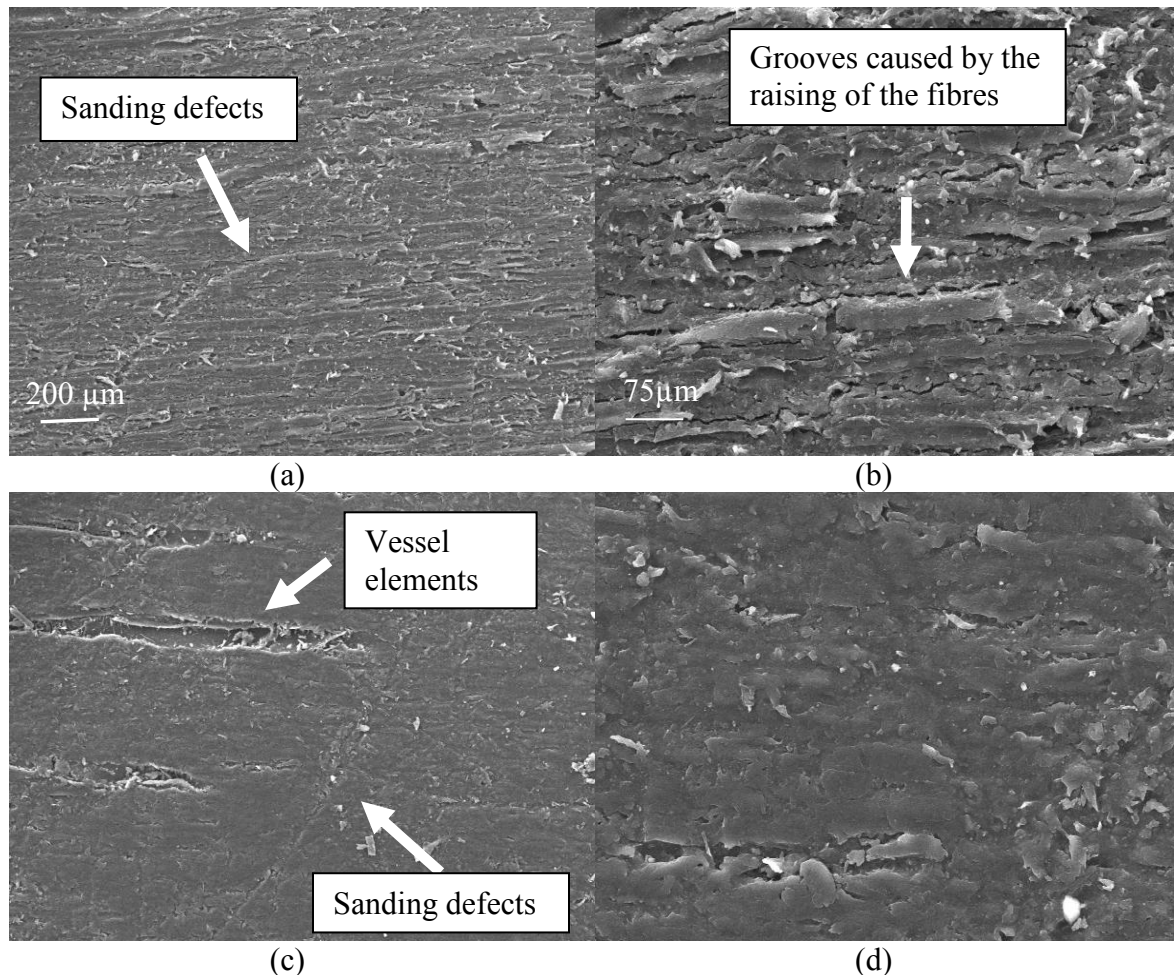
Fig. 5. Lumber samples stained with a water-based stain (a, b) vs. a solvent-based stain (c, d)
