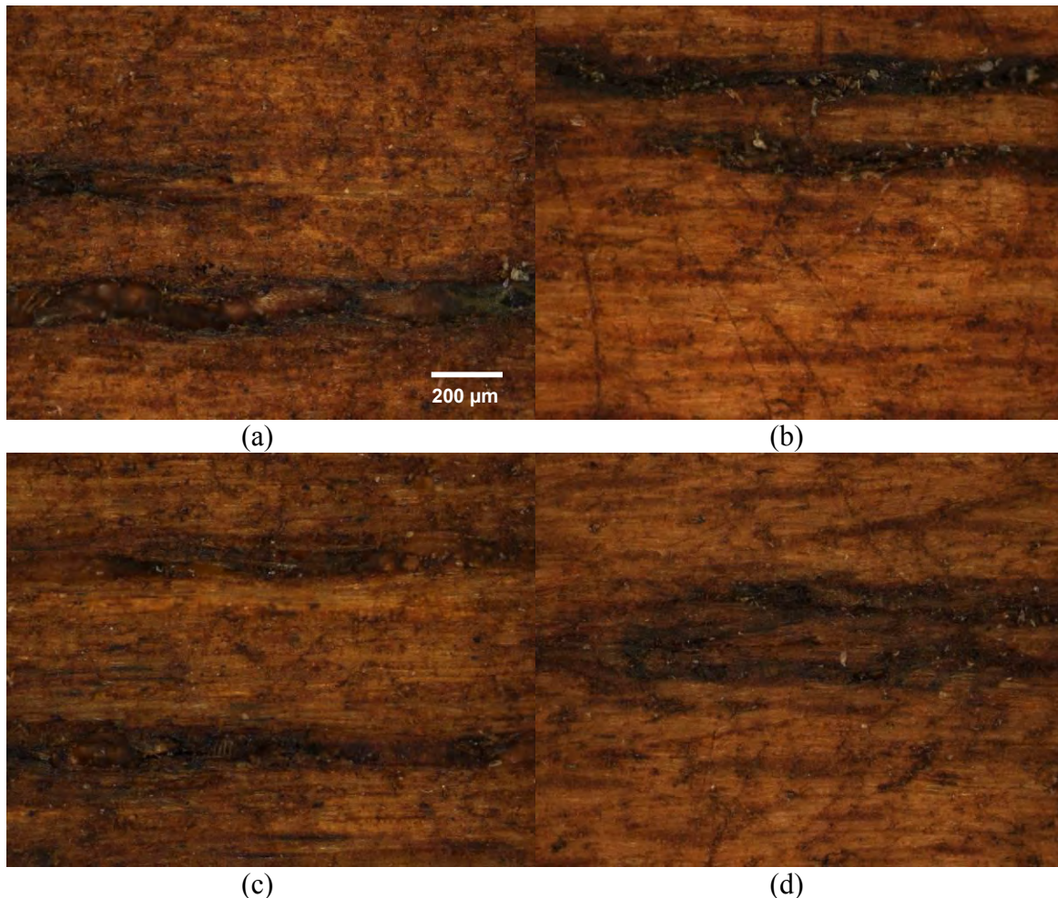
Fig. 3. Images of stained surfaces (a) lumber with a water-based stain; (b) lumber with a solvent-based stain; (c) veneer with a water-based stain; (d) veneer with a water-based stain
