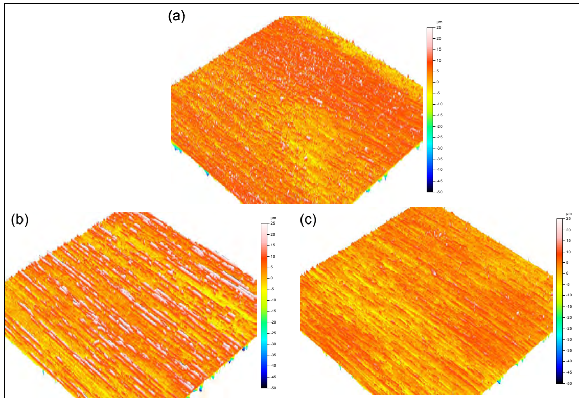
Fig. 7. 3D Renderings of profilometric measurements on sanded veneer without finishing products (a); with a water-based stain (b); with a solvent-based stain (c). Color scale goes from -50 \mu\text{m} to 25 \mu\text{m} Surface dimensions: 20 x 20 mm
