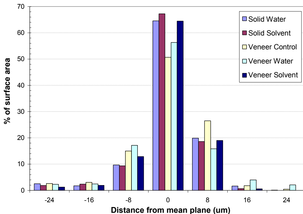
Fig. 9. Histograms of the heights on yellow birch solid and veneer samples
