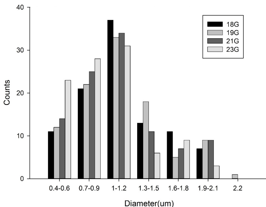
Fig. 6. Distribution of fiber diameters obtained at different needle gauges at solution concentration of 20 wt% (Chang et al. 2014)
