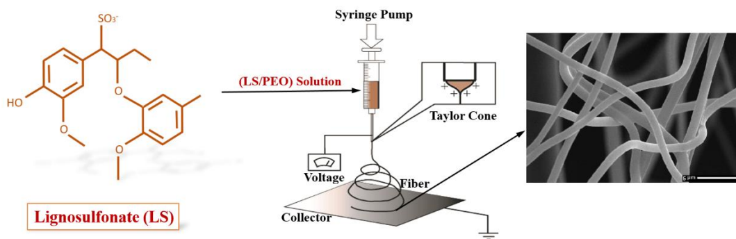
Fig. 1. Schematic of the electrospinning apparatus to produce lignosulfonate fibers
