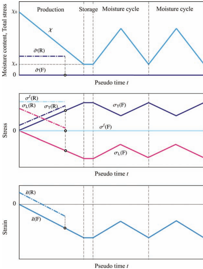
Figure 3. (Top) Applied moisture content and overall stress history to mimic the production of the sheet and subsequent moisture cycling experiments, for the free drying condition ((F), solid line) and the restrained drying condition ((R), dash-dotted line). (Middle) Resulting evolution of the stresses in the fibres as predicted by the hygro-elastic reference model for the free ((F), solid line) and restrained ((R), dash-dotted line) drying conditions: stress in the free-standing fibre segment, \sigma^f , and in the fibre parts which compose the bond, in longitudinal direction, \sigma_L , and transverse direction, \sigma_T . (Bottom) Resulting overall (sheet-scale) strain of the network, \bar{\epsilon} , again for the free and constrained condition.
