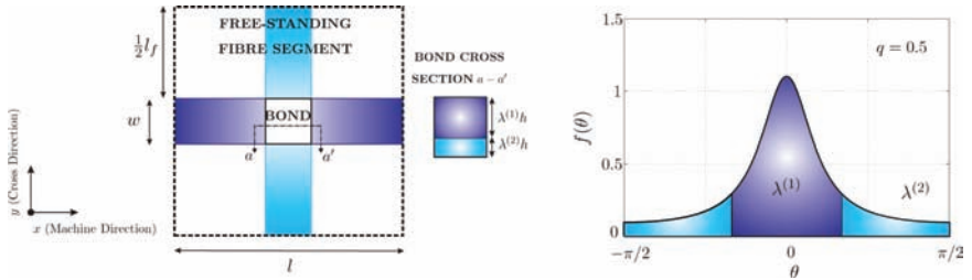
Figure 2. Sketch of the micro-structural model employed in our study: ( left ) geometry of a unit cell of the idealised periodic network considered and ( right ) fibre orientation distribution and its translation into relative thicknesses of the MD and CD fibres.
