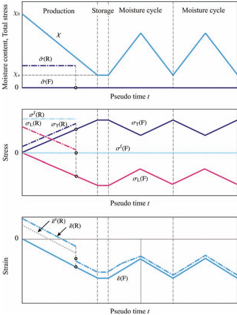
Figure 4. (Top) Moisture and stress history applied to the model with activation – identical to that used for the reference model (cf. Figure 3), but repeated for clarity. Solid lines, marked with (F) refer to free drying and dash-dotted lines, marked (R), to restrained drying. (Middle) Predicted evolution of the stresses in the free-standing and bonded parts of the fibres; these, too, coincide with those of the reference model, although the tensile stress in the free-standing fibre parts now results in activation/plasticity. (Bottom) Resulting overall (sheet-scale) strain evolution of the network. The hygro-elastic response of Figure 3 is shown as a dotted line (and marked \bar{\epsilon}^e ) for comparison.
