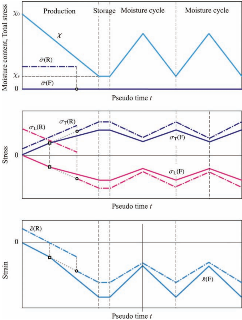
Figure 6. (Top) Applied moisture and stress history – repeated for clarity. (Middle) Evolution of the stresses in the free-standing and bonded parts of the fibres as predicted by the model with micro-buckling for the free drying and restrained drying conditions (solid and dash-dotted lines, respectively). The response of the reference model is also shown, by dotted lines, for comparison. (Bottom) Resulting overall (sheet-scale) strain evolution of the network, together with that of the reference model.
