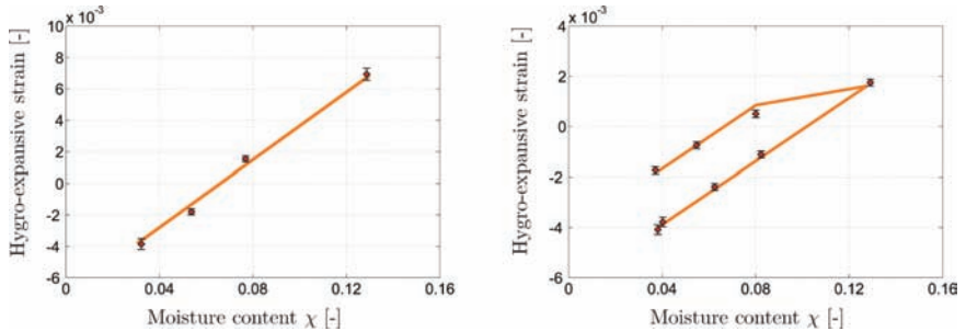
Figure 8. Comparison of the predicted hygro-expansive behaviour as a function of moisture content with experimental data presented in [7], for ( left ) freely-dried hand-sheets and ( right ) restrained-dried hand-sheets. The curves represent the predicted response, the markers denote the experimental data for untreated, virgin fibres.
