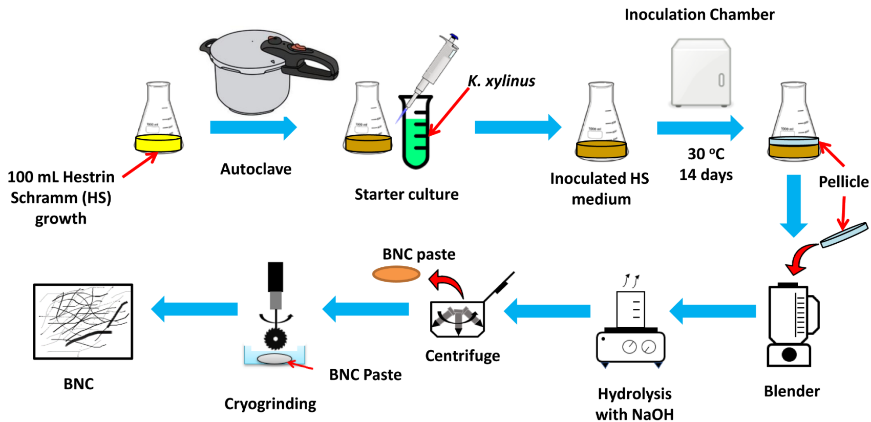
Fig. 1. Synthesis and preparation process of bacteria nanocellulose (BNC)
