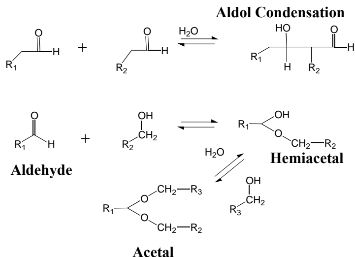
Scheme 1. Aldehyde coupling by the aldol condensation reaction and aldehyde reactions with alcohols to form hemiacetal and acetal linkages
