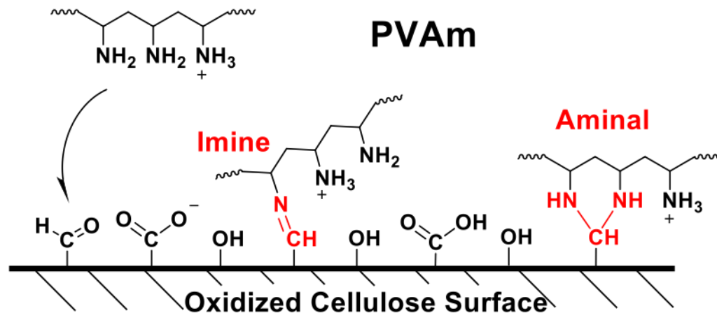
Scheme 2. Grafting reactions for PVAm on oxidize cellulose. Figure adapted from Yang et al. (2018b).
