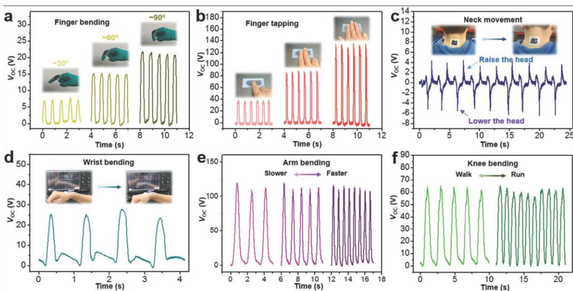
Fig. 2. CM-TENG-based self-powered biomechanical sensor for monitoring human body movements: a) finger bending, b) finger tapping, and c) neck movement. Generated VOC of the CM-TENG under different bending frequency of d) wrist, e) arm, and f) knee (Cao et al. 2020)
