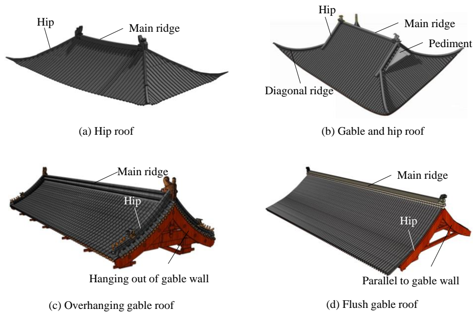
Fig. 15. Chinese ancient wood architectures
