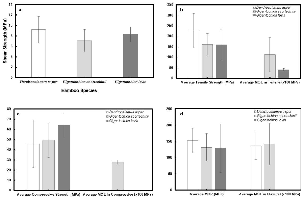
Fig. 4. Average shear, tensile, compressive, flexural strength of bamboo from various bamboo species
