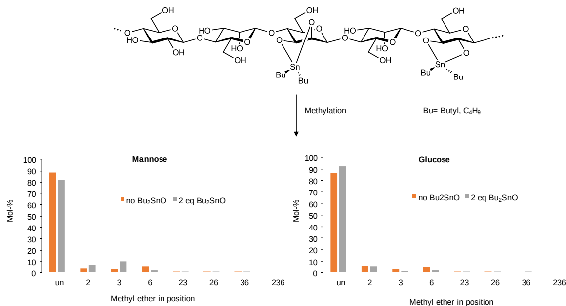
Fig. 17. Methyl pattern obtained by tin-mediated methylation of konjac glucomannan (M-KGM 2) in comparison with a reference experiment under the same conditions, but without \text{Bu}_2\text{SnO} (M-KGM 1, see Online Resource Table A1). Molar portions are given separately for mannose (a) and glucose (b), both normalized to 100 % (redrawn from Raßloff et al. 2018)
