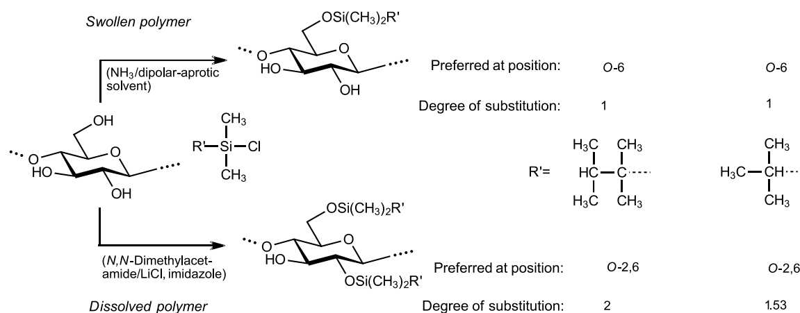
Fig. 4. Regioselectivities of trialkylchlorosilanes depending on the activation state of cellulose. References: Thexyldimethylsilyl ether (Klemm and Stein 1995; Koschella and Klemm 1997), tert-butyldimethylsilyl ether (Heinze et al. 2008)
