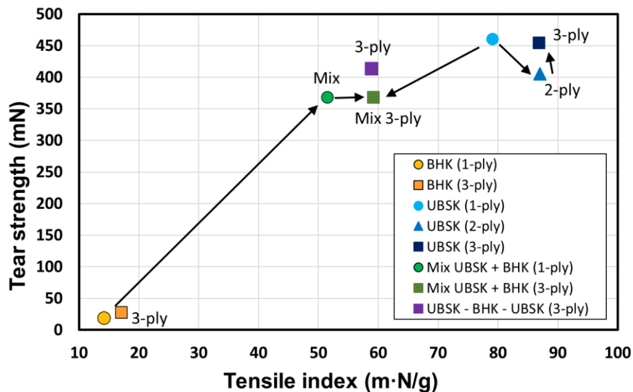
Fig. 4. Comparison of the tear strength as a function of the tensile index of single-ply and multi-ply papers formed from UBSK (● one-ply, ▲ two-ply, ■ three-ply), BHK (● one-ply, ■ three-ply) or mixed UBSK-BHK pulps (1:1, ● one-ply, ■ three-ply). Three-ply paper where only the internal layer was formed from BHK pulp has been marked in violet (■). The grammage of all papers was 150 g/m 2 .
