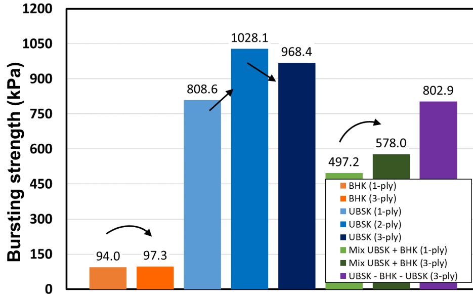
Fig. 9. Comparison of the bursting strength values for all variants of paper samples (single- and multi-ply papers)
