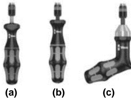
Fig. 2. Torque screwdriver (a) 0.1 < 1.2 N.m, (b) 1.2 < 3.0 N.m, (c) 3.0 < 6.0 N.m
