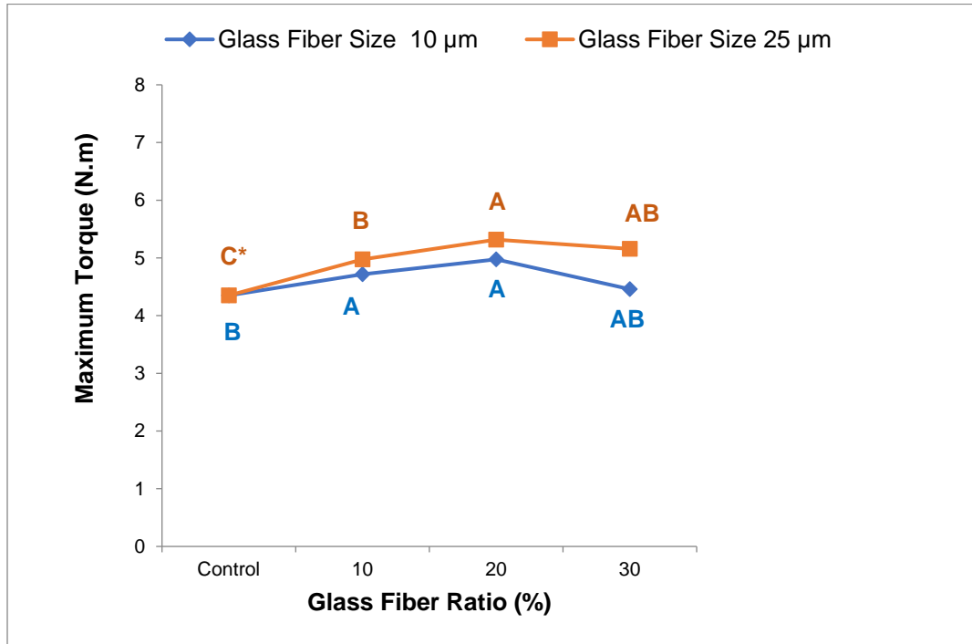
Fig. 5. Comparison of average maximum torque value according to glass fiber ratio in each glass fiber size (* Means followed by a common letter are not significantly different at the 5% level) (LSD = 0.3022)
